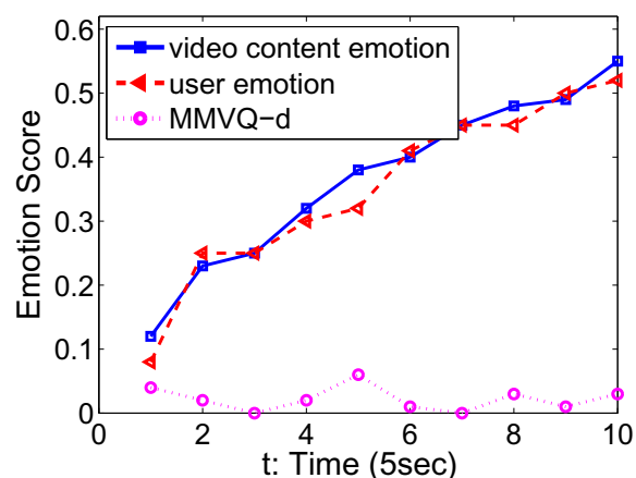
Fig. 7. Mood matching for video QoE after adjustment.
