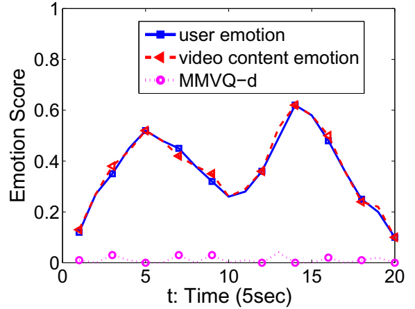
Fig. 4. MMVQ metric.
