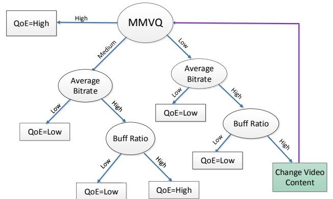
Fig. 5. The decision tree-based adjustment model for video QoE.
