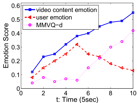
Fig. 6. Mood matching for video QoE before adjustment.
