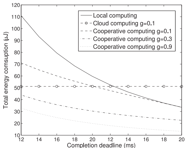
Fig. 6. Total energy consumption versus completion deadline.
