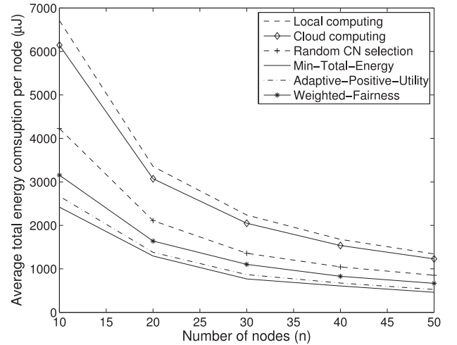
Fig. 7. Average total energy consumption per node for L = 1,024 bits.
