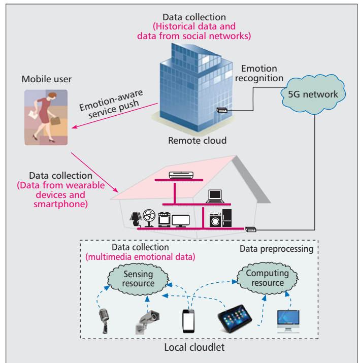
Figure 1. The proposed EMC architecture.
