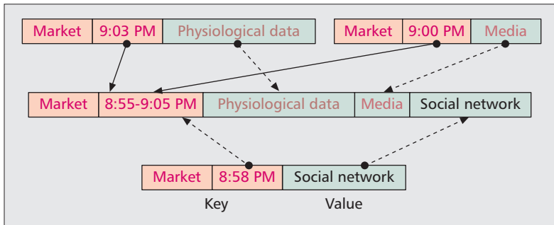
Figure 4. Illustrative example of a data structure for data integration.
